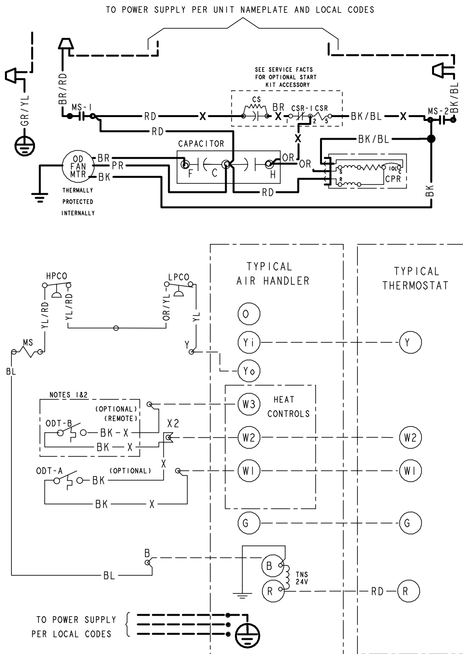
Figure 3. 060 Models
