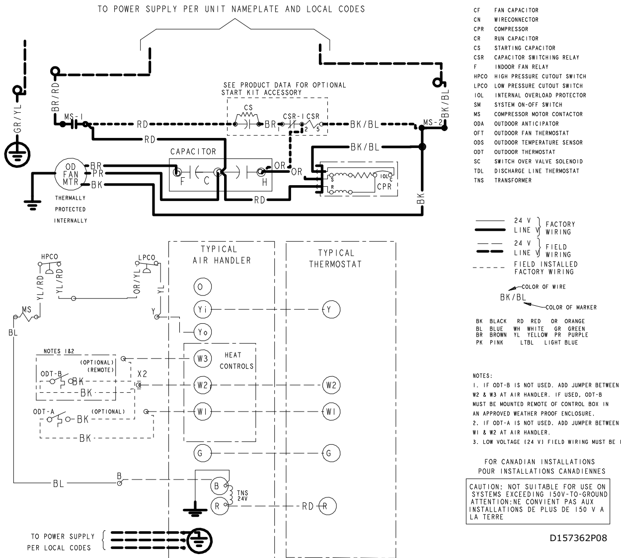
Figure 1. 018 — 048 Models
