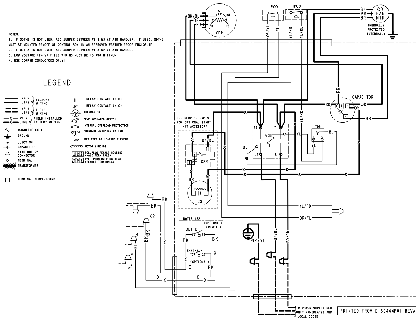
Figure 4. Schematic: 5 Ton Model
