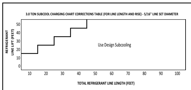
Figure 3. Subcool Charging Corrections – 4.0 Ton
