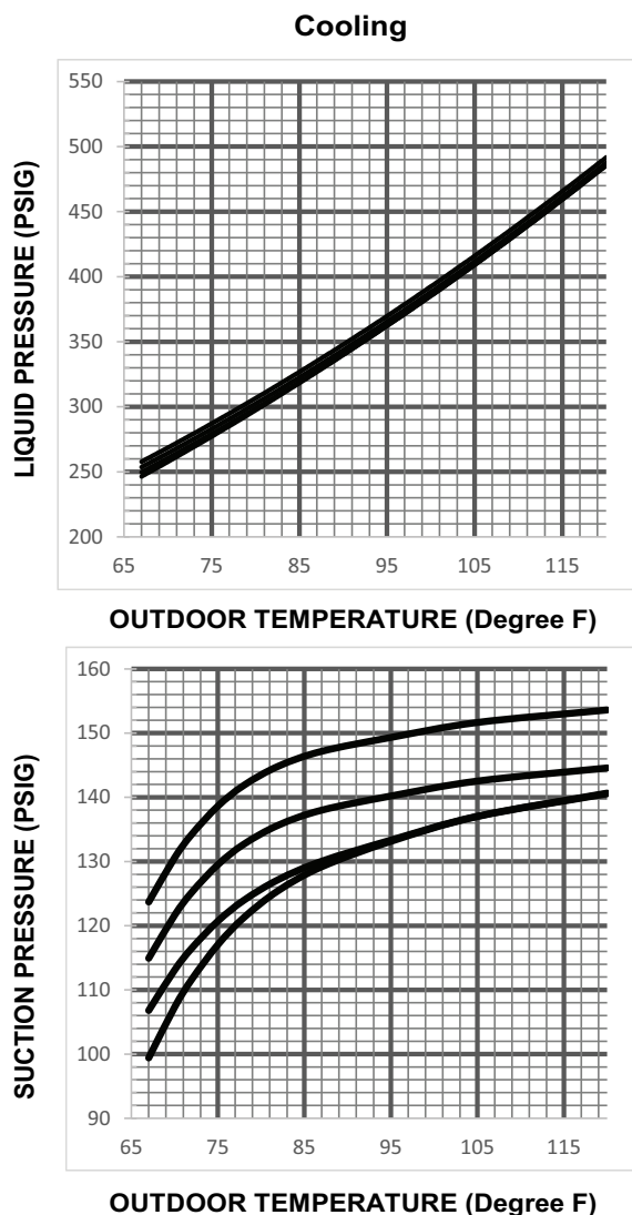
Figure 15. 4 Ton AC (X48 Models)
