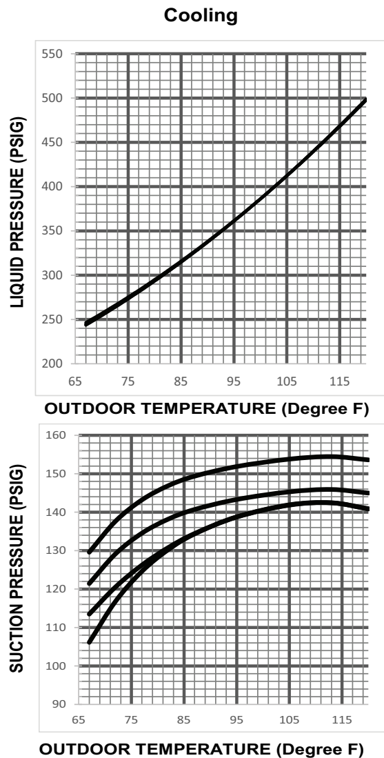
Figure 13. 2 Ton AC (X24 Models)
