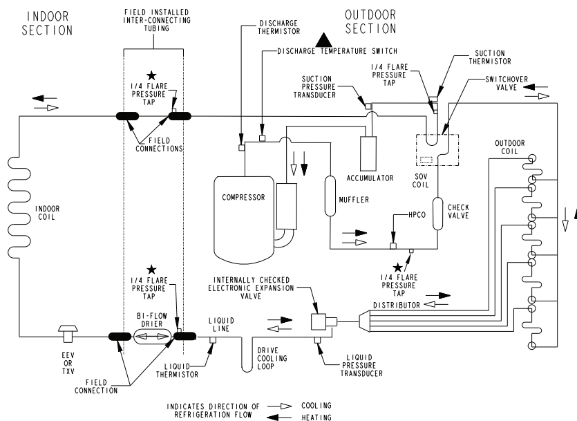
Figure 5. 2 Ton and 3 Ton HP (X24 and X36 Models)
