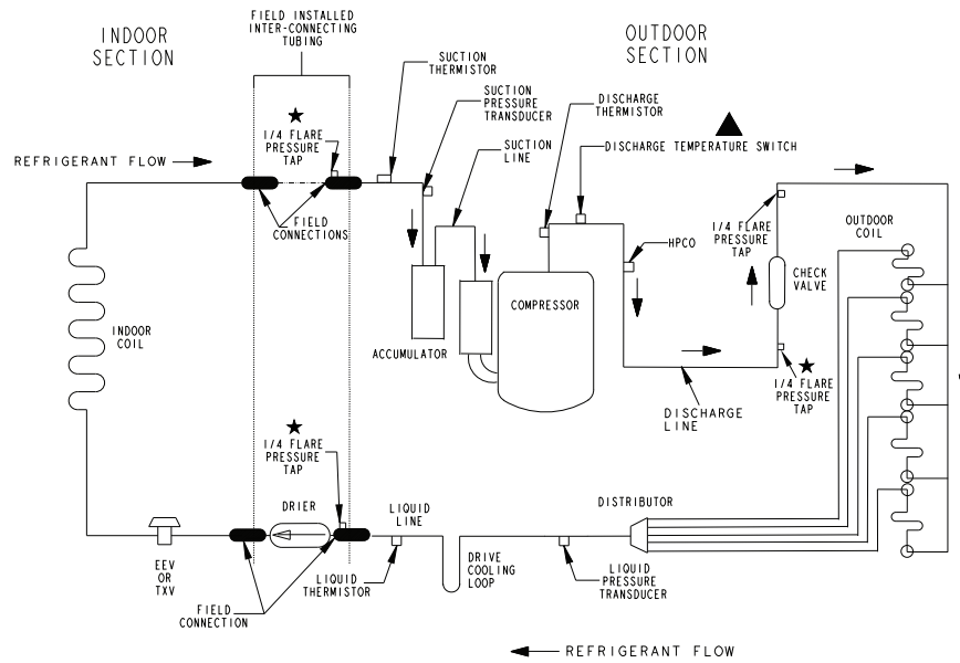
Figure 7. 2 Ton and 3 Ton A/C (X24 and X36 Models)
