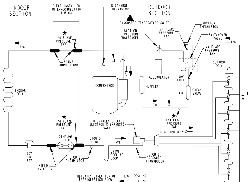
Figure 6. 4 Ton and 5 Ton HP (X48 and X60 Models)
