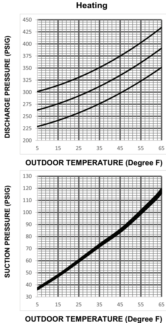
Figure 12. 5 Ton HP (X60 Models)
