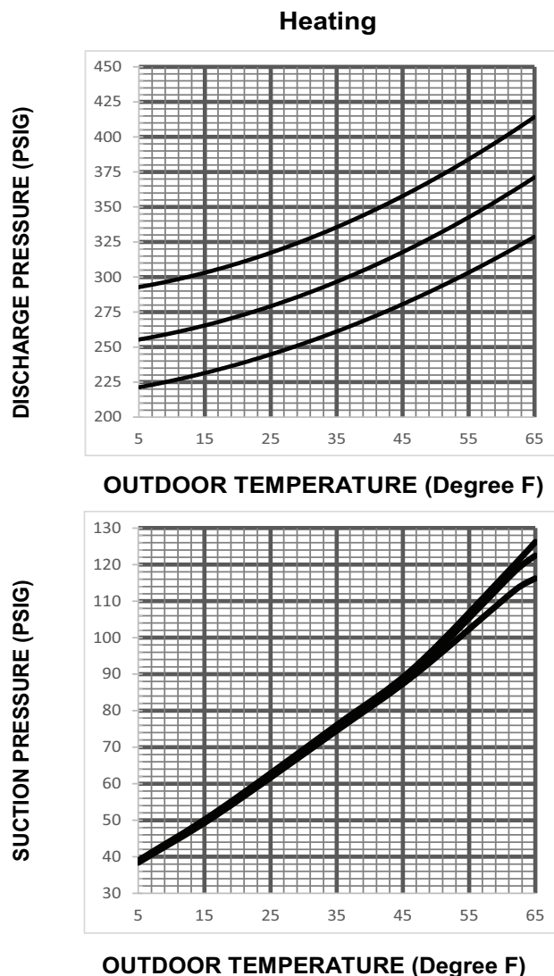
Figure 11. 4Ton HP (X48 Models)
