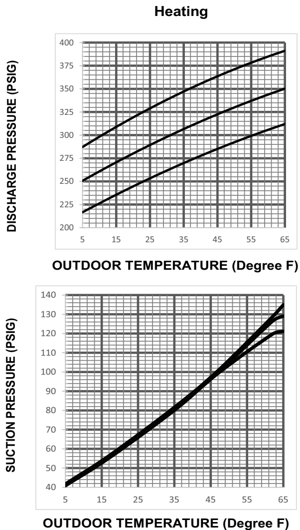
Figure 9. 2 Ton HP (X24 Models)
