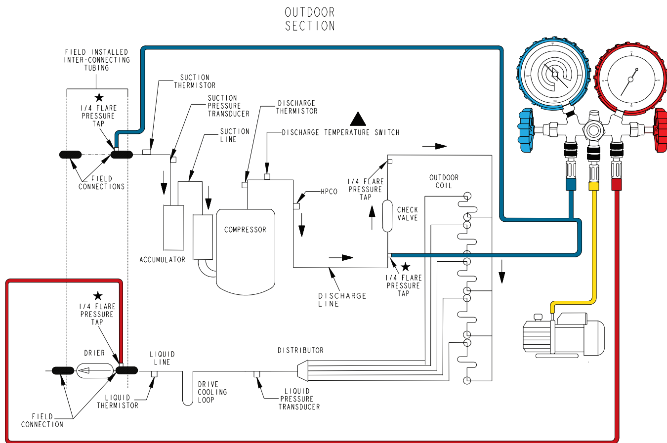
Figure 17. Evacuating Outdoor Unit
