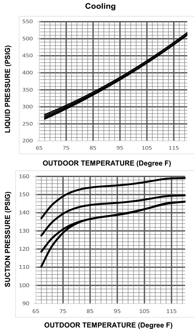
Figure 14. 3 Ton AC (X36 Models)
