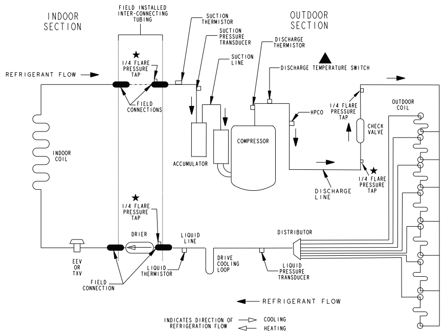
Figure 8. 4 Ton and 5 Ton A/C (X48 and X60 Models)
