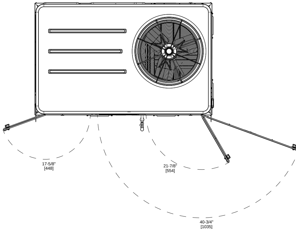
Figure 23. B.0 cabinet
