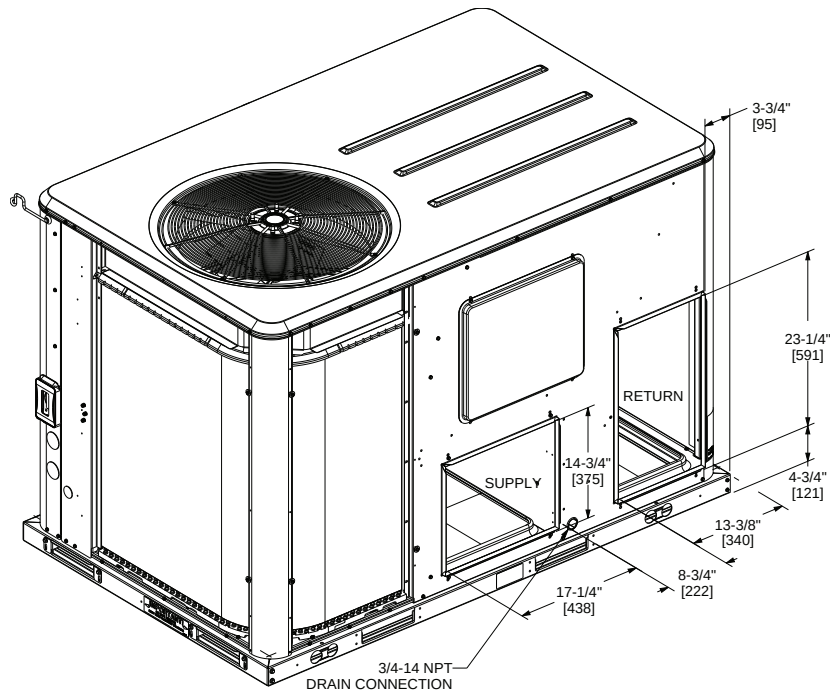
Figure 19. A.0 cabinet – unit clearance and roof opening
