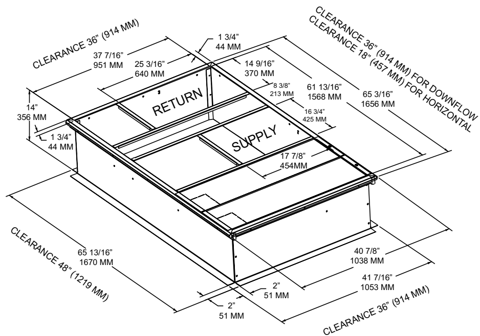
Figure 21. A.O cabinet – downflow duct connections, field fabricated
