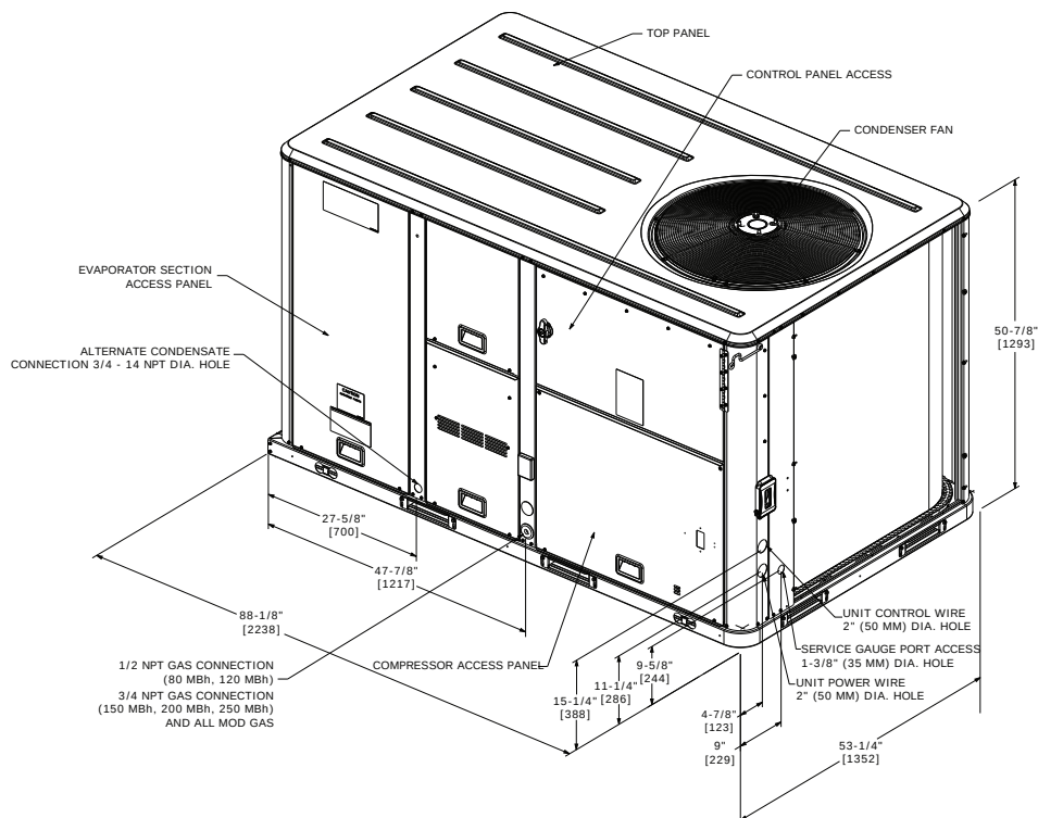
Figure 23. B.0 cabinet
