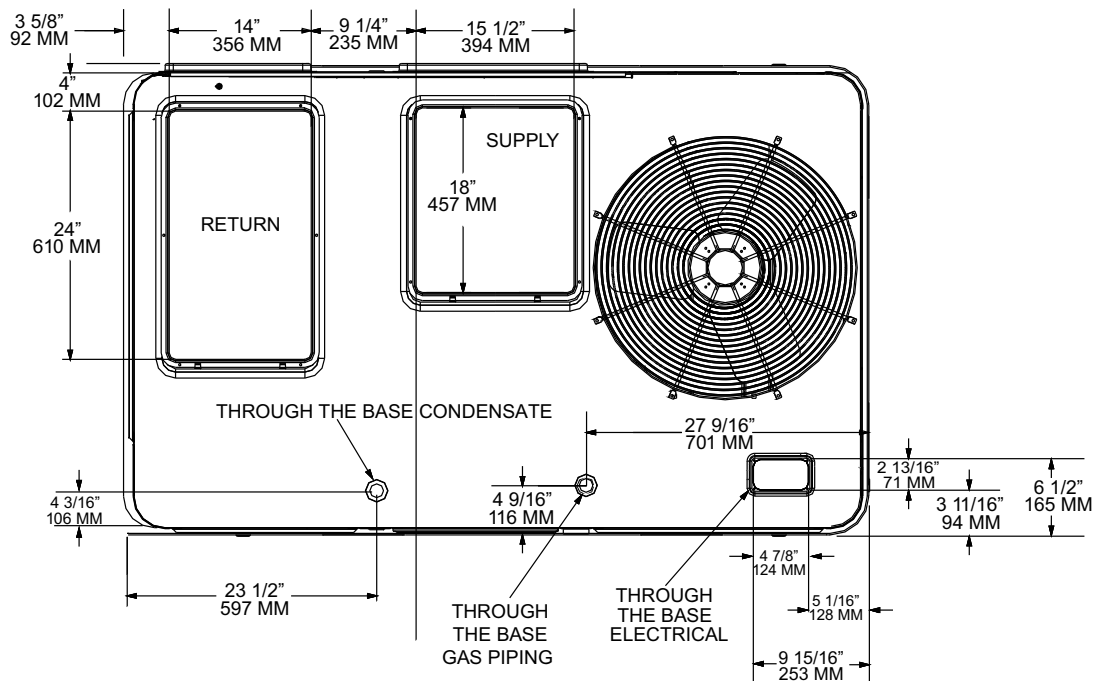
Figure 17. A.O cabinet – downflow airflow supply/return, through-the-base utilities
