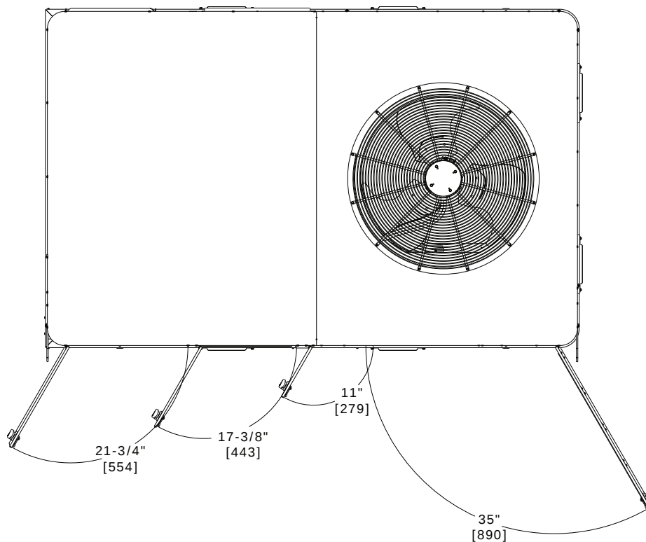
Figure 35. C.O cabinet – swing diameter for hinged door(s) option
