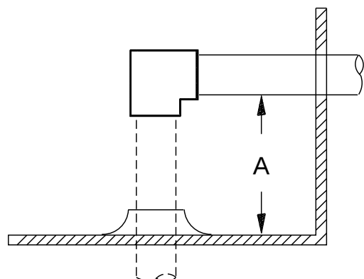
Figure 46. Gas pipe height
